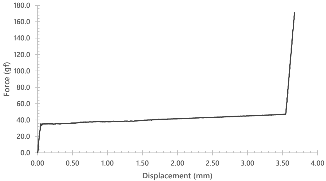
Kailh Box Taro Ice Cream Pro (Upstroke)
